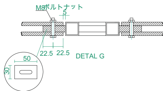
DETAL H
