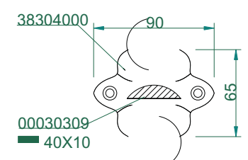
DETAIL A 1:4
