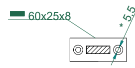
DETAIL C 1:4
