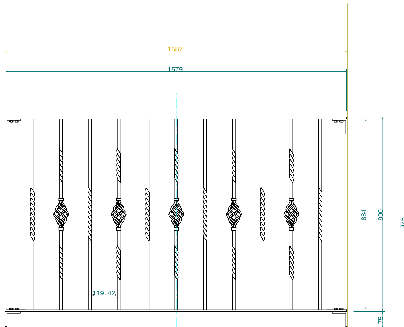
(12)手摺2F x2
